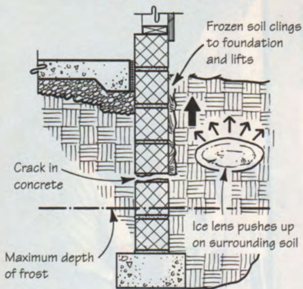
Figure 1. As the soil around an unheated building freezes and expands, it can “grip” the foundation and lift the wall apart (left). Although block walls are particularly susceptible, poured concrete walls can also be damaged (above).
